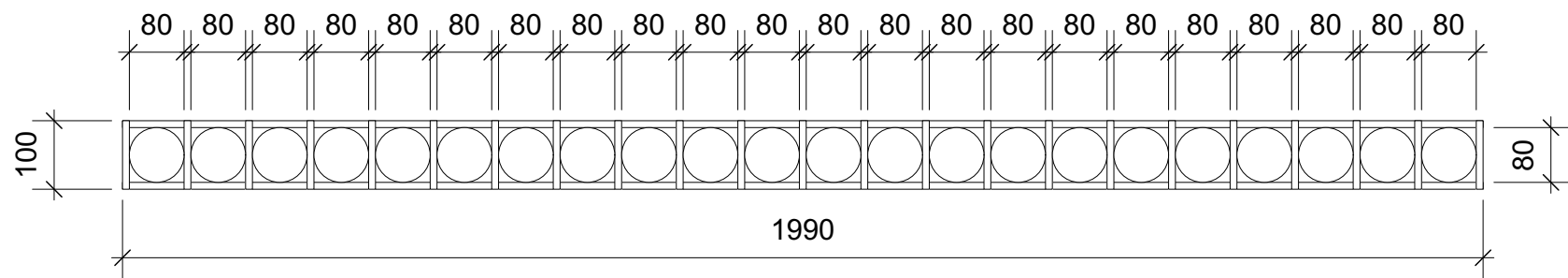
SECTION A-A / SCALE 1:10
