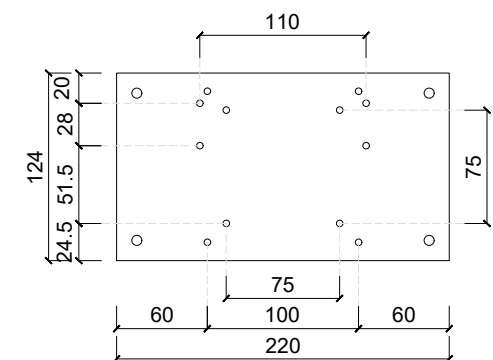
DETAIL H-2 WALL MOUNT KIT (FRONT)
