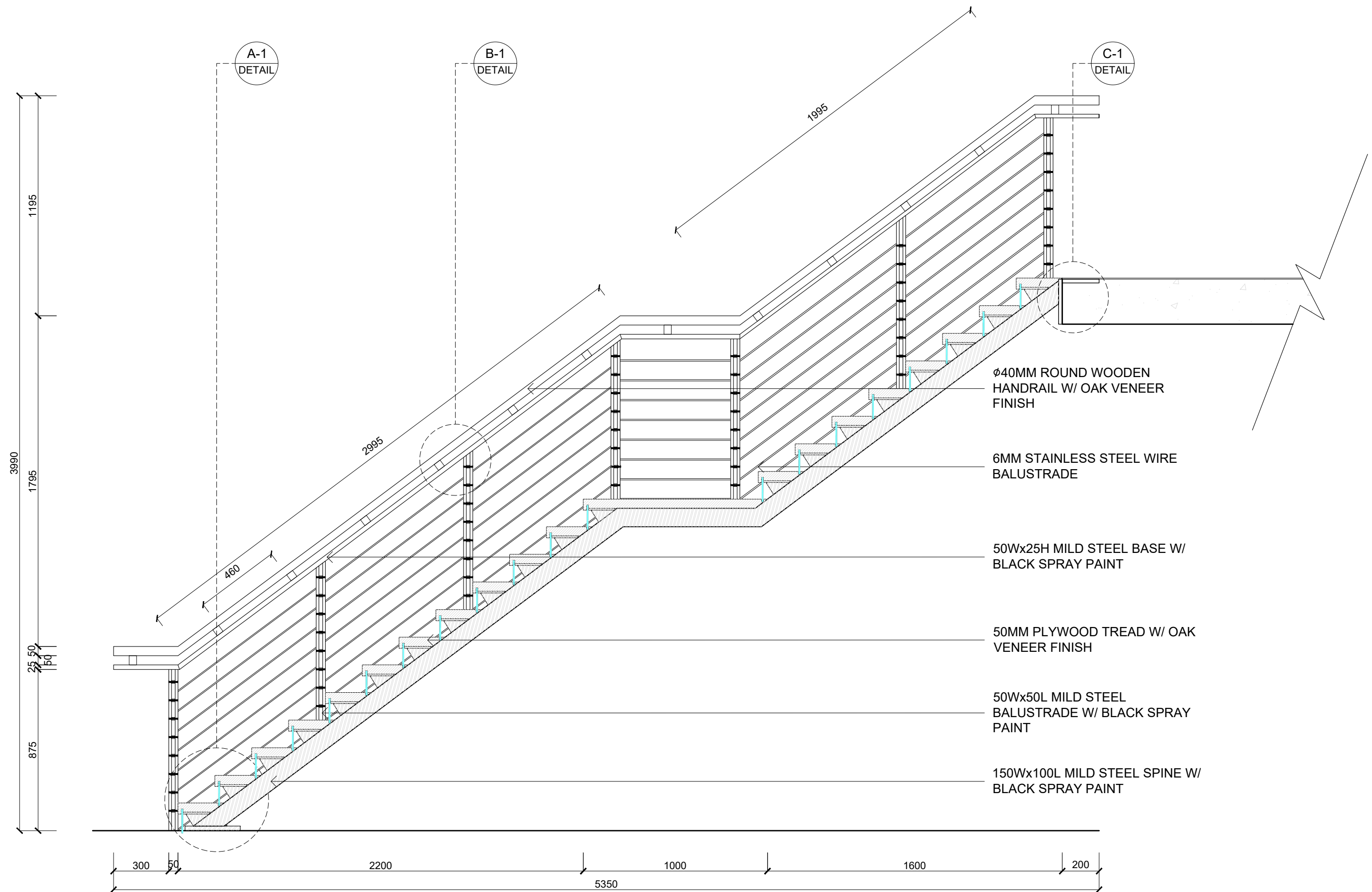
SECTION S-1 MAIN STAIRCASE
