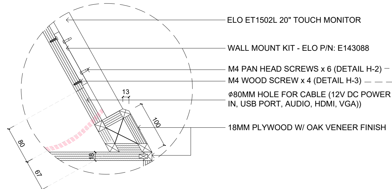
DETAIL H-1 TOUCH MONITOR
