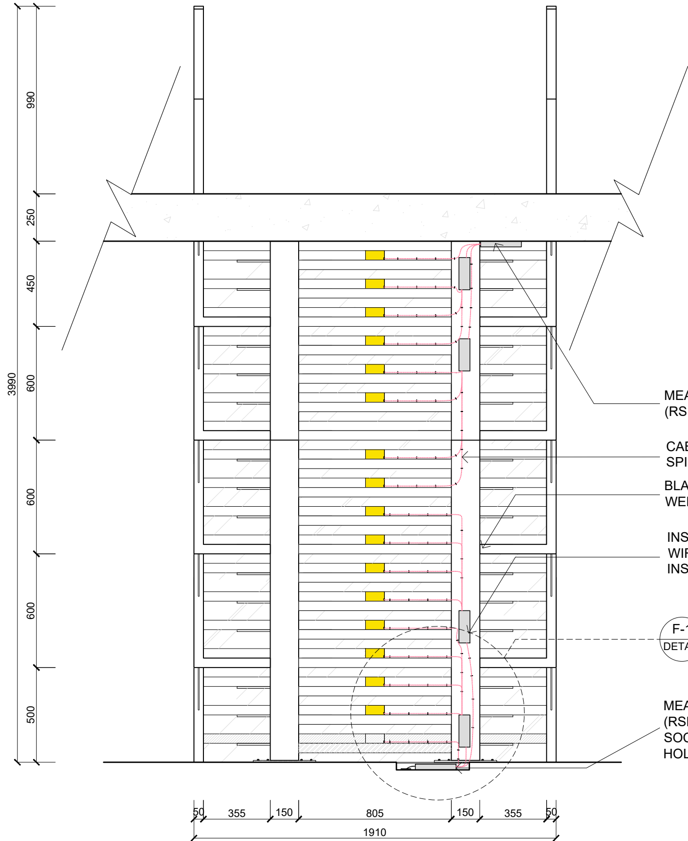
SECTION S-3 MAIN STAIRCASE
