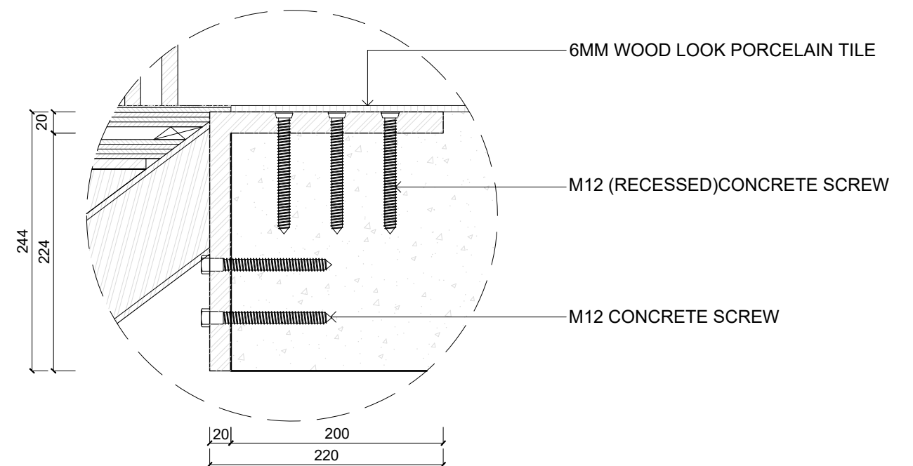
DETAIL C-1 1:5 MAIN STAIRCASE STRUCTURE (CONNECTING TO PLATFORM)
