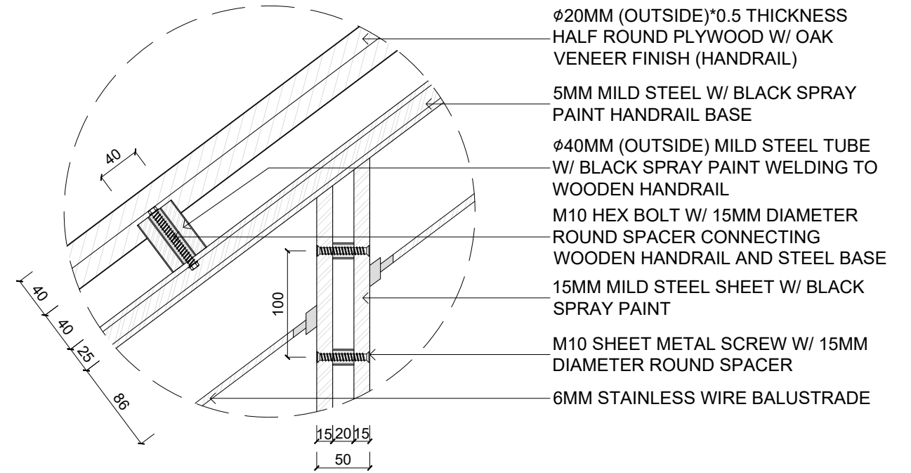
DETAIL B-1 1:5 MAIN STAIRCASE HANDRAIL
