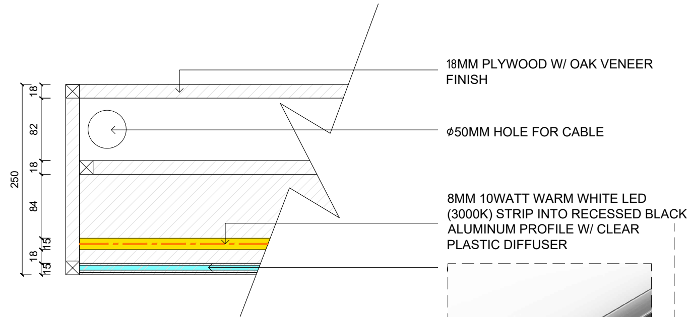
SECTION S-7 MATERIAL LIBRARY - DISPLAY WINDOW
